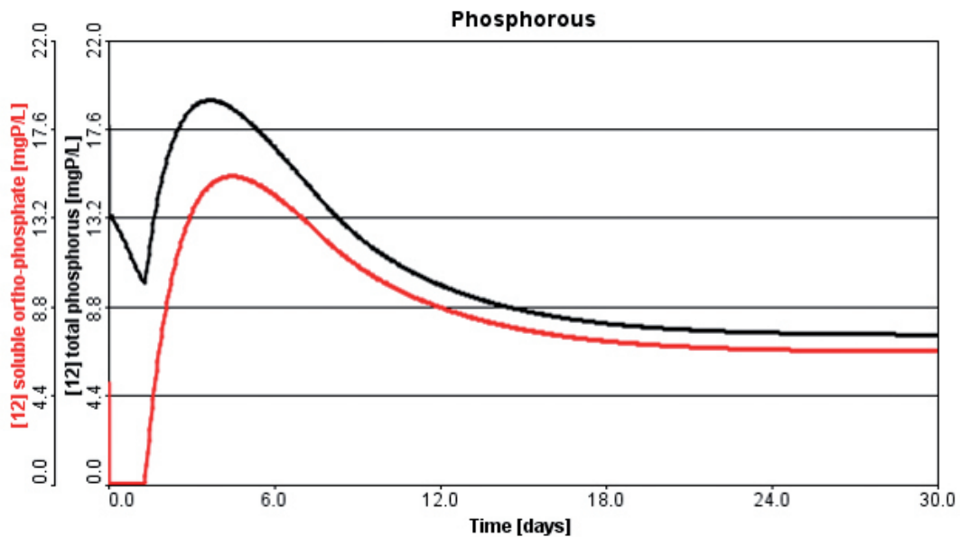
Figure 17 Effluent phosphorus concentration (compiled by the author)
