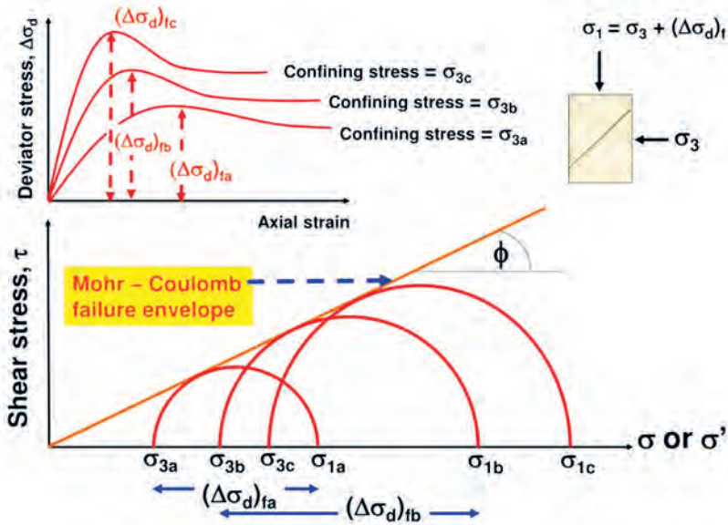
Figure 13. Series of three triaxial tests at increasing confining stress [6]
