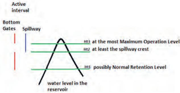
Figure 5. Outlets operation rules [8]
