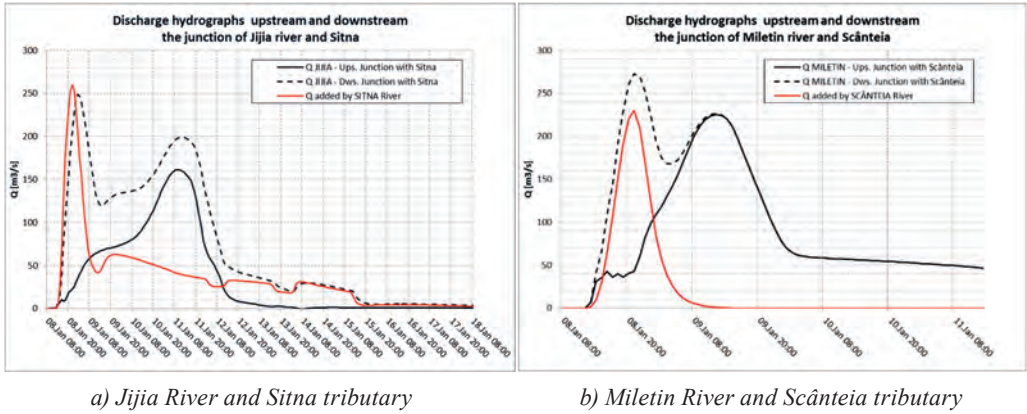
Figure 15. Discharge hydrographs upstream and downstream the confluence of the main river with a tributary [8]
