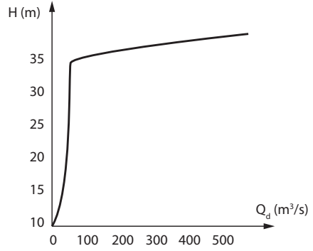
Figure 3. Elevation-outflow curve [11]
