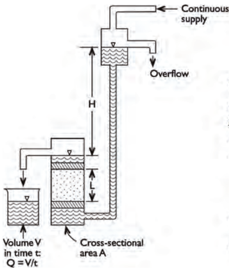
Figure 12. Darcy's Law applied to laboratory constant head test [14]
