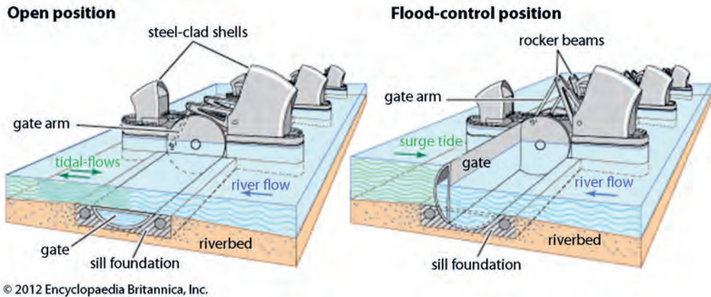
Figure 3. Thames barrier, London – Functional sketch [8]
