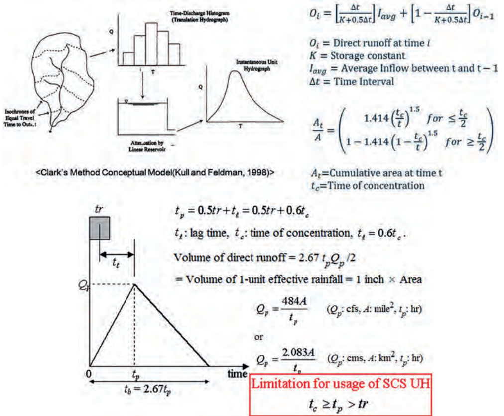
Figure 13. The Snyder UH (top panel) and the SCS SUH (bottom panel) [38]
