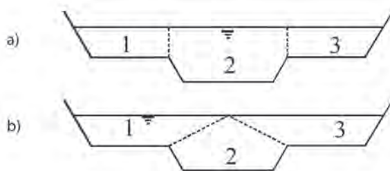
Figure 4. Possible divisions of the compound channel into subsections in the DCM; a) division using vertical; b) diagonal plains [16]
