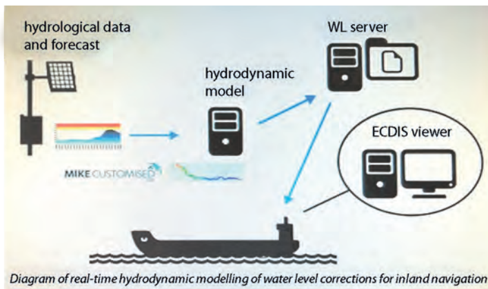
Figure 16. Diagram of real time hydrodynamic modelling of water level (MIKE HIDRO River modelling package)
