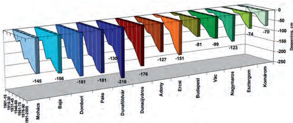
Figure 17. Lowering of the Danube stages along the Hungarian reach [2]
